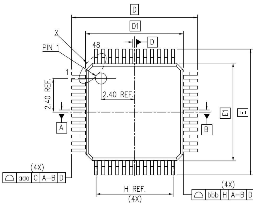
Figure 22 LQFP48 Package Diagram
